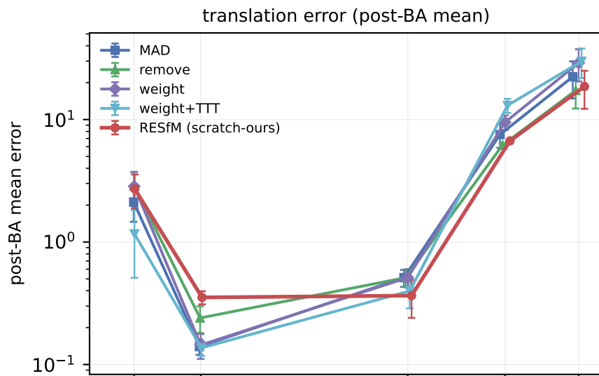
trained on MegaDepth (OOD eval)
